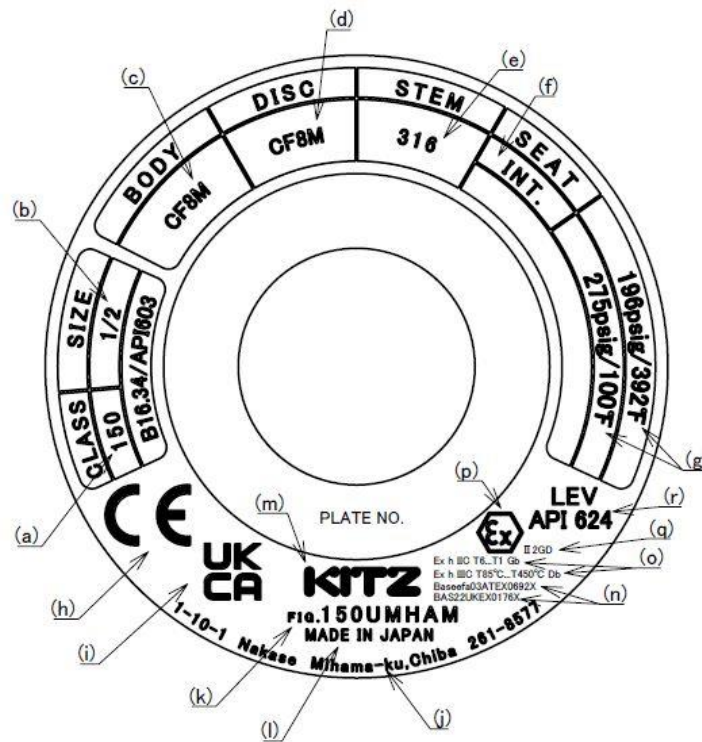
Fig.1 Example of Gate valves UMHA series
