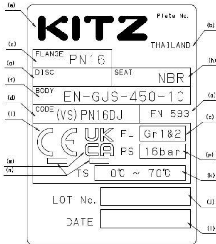
Fig.3 Example of Butterfly Valves nameplate
