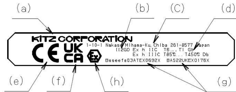
Fig.5 Example of Gate valves, Glove valves, Check valves and Ball valves nameplate
