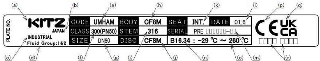
Fig.1 Example of Gate valves, Globe valves and Check valves
